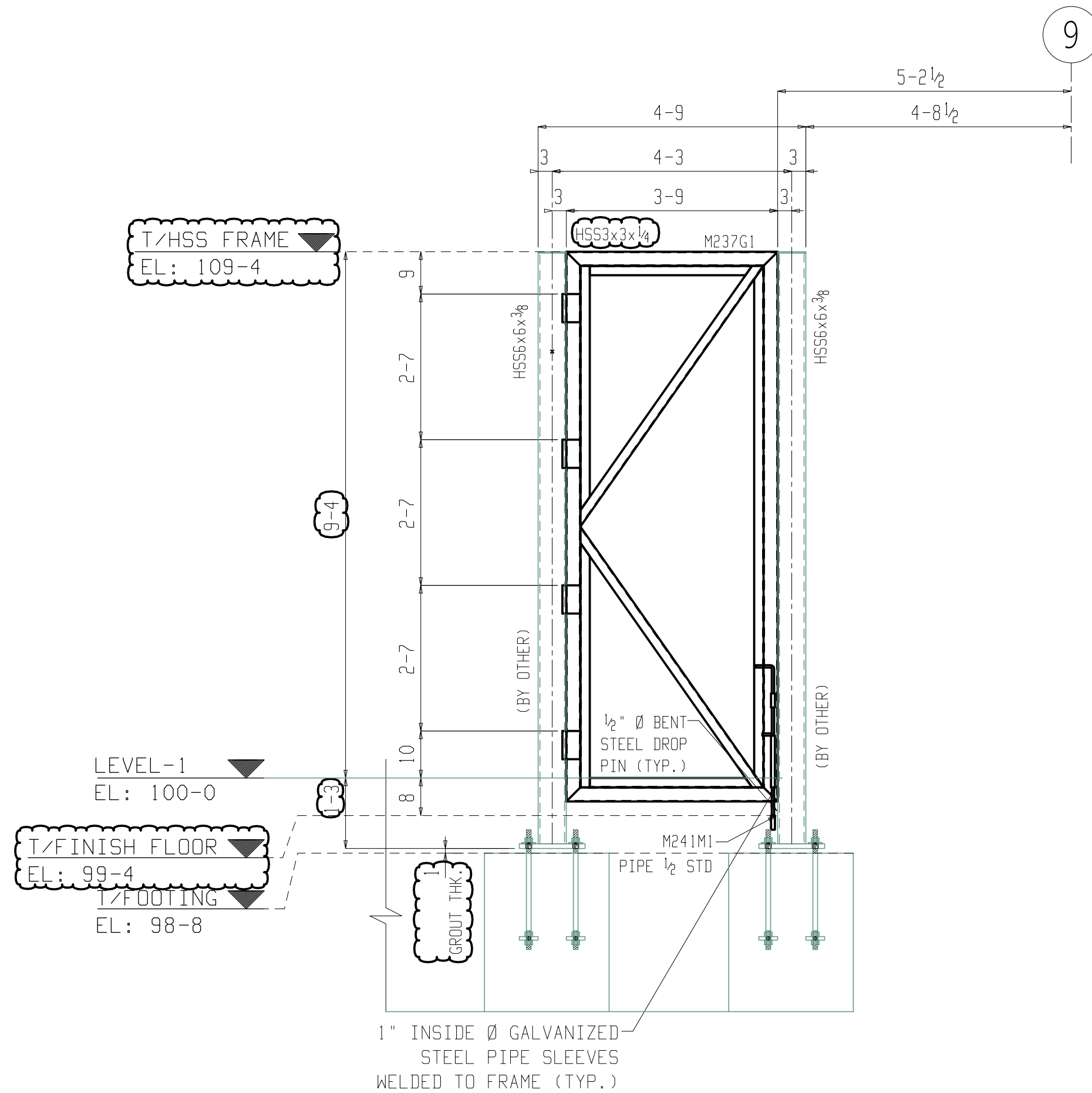
5 TRASH ENCLOSURE ELEVATION ME159 (REF DWG: F5/AS1.23))
