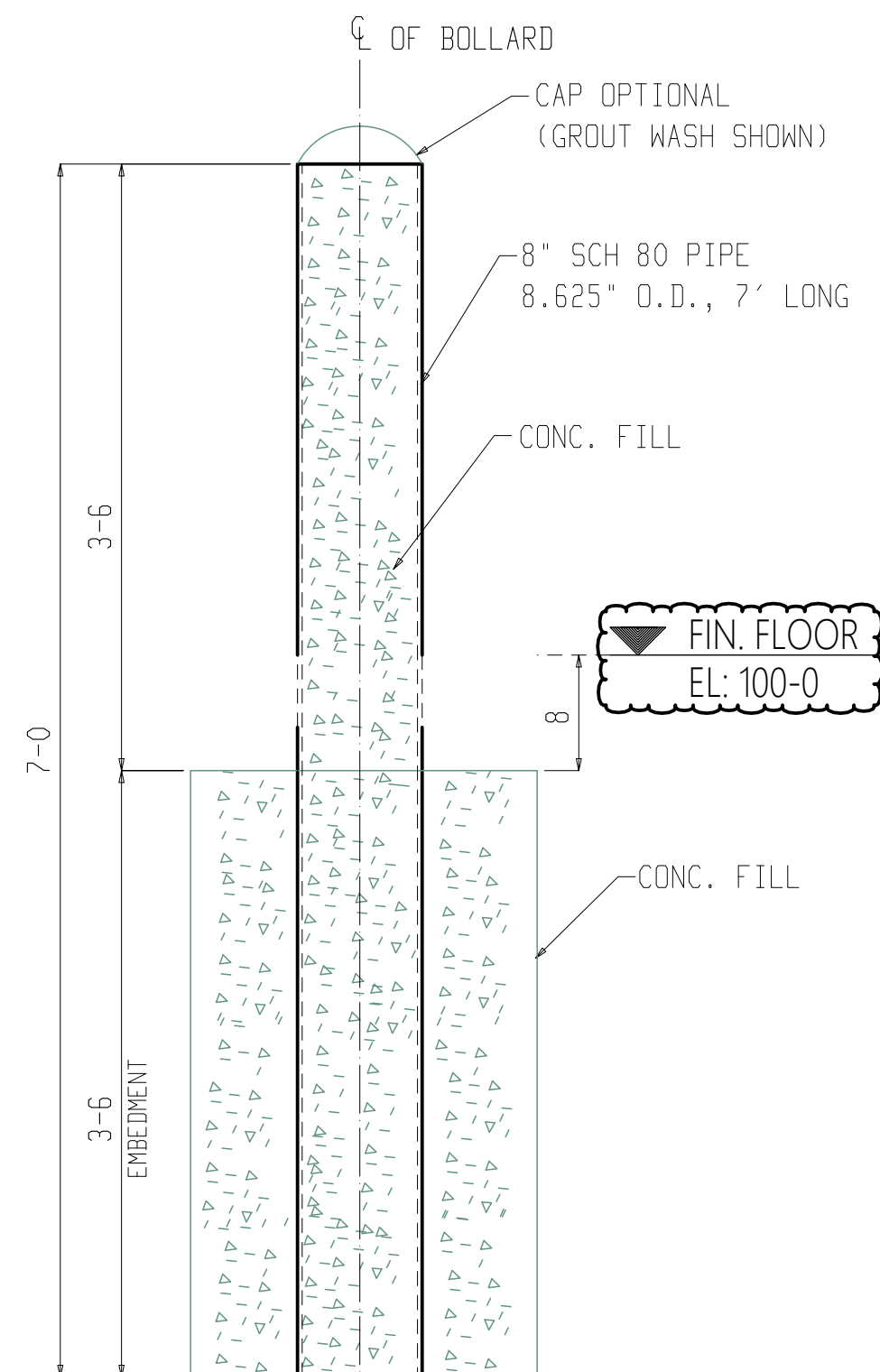
TYPICAL BOLLARD SECTION (REF. SEC.D/AS1.25)
