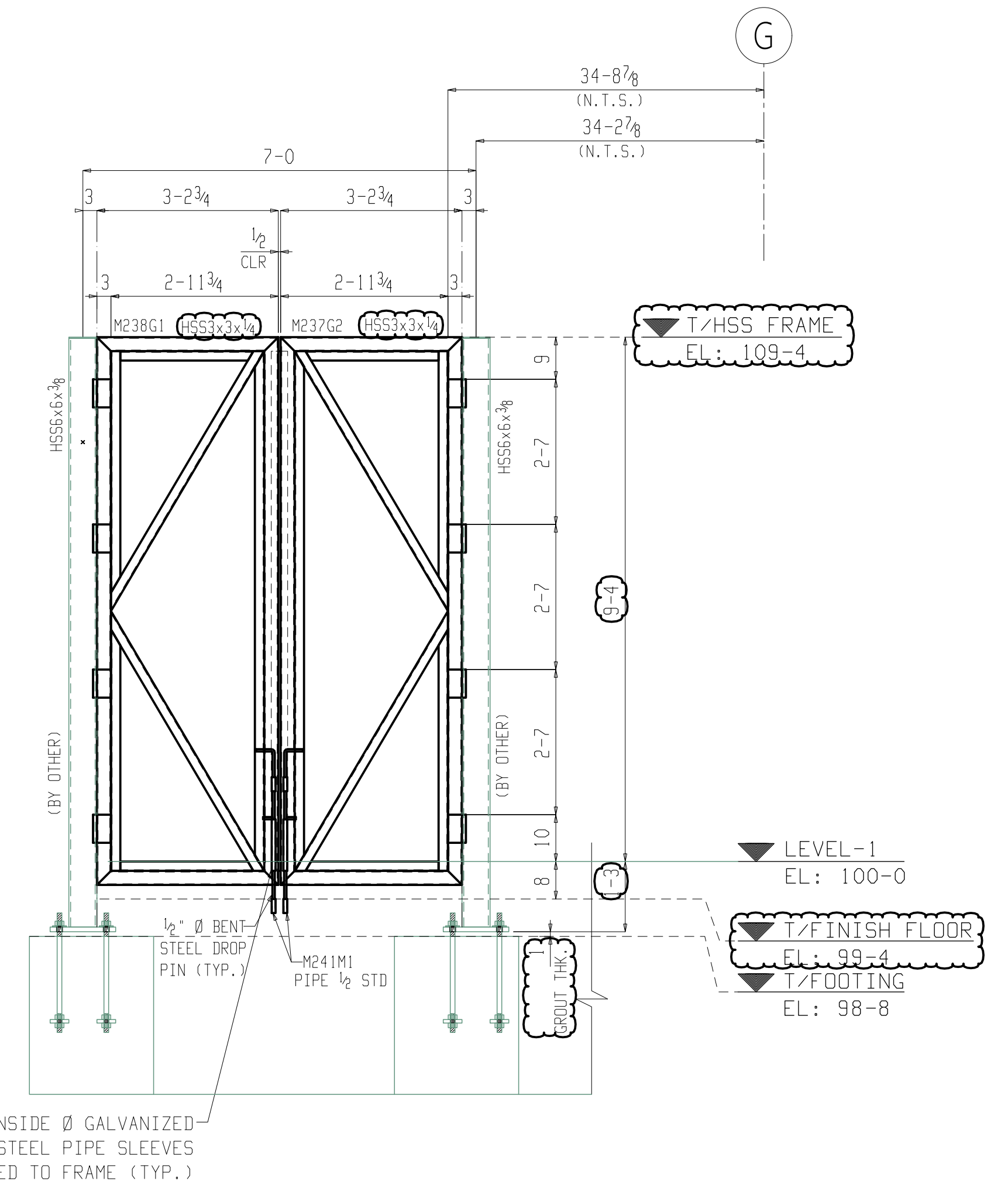
4 TRASH ENCLOSURE ELEVATION ME159 (REF DWG: F2/AS1.23))
