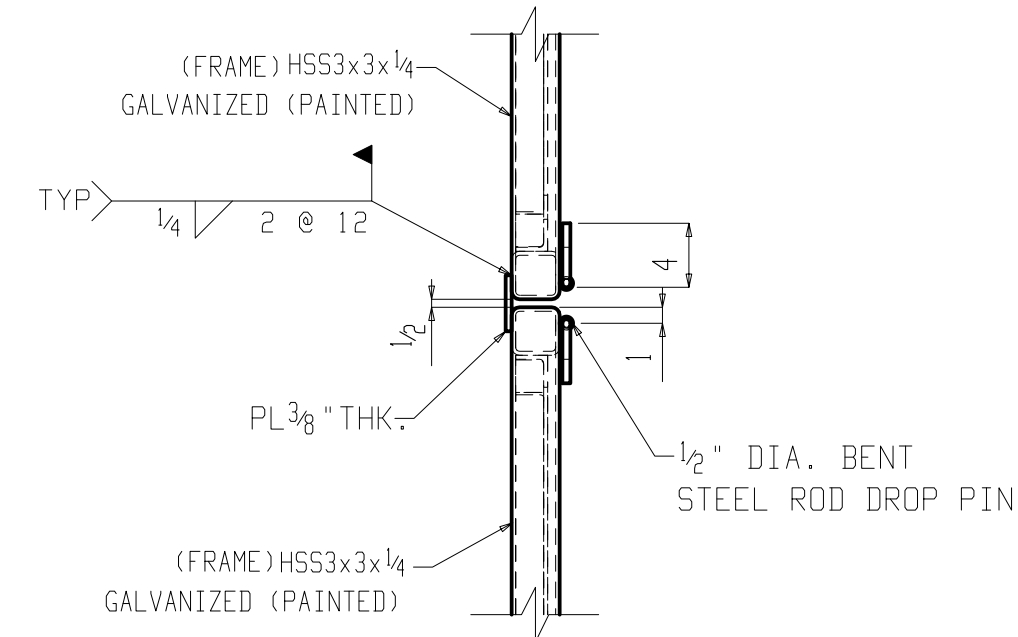
3 DETAIL VIEW ME159 (REF DWG: (A3/AS1.23))
