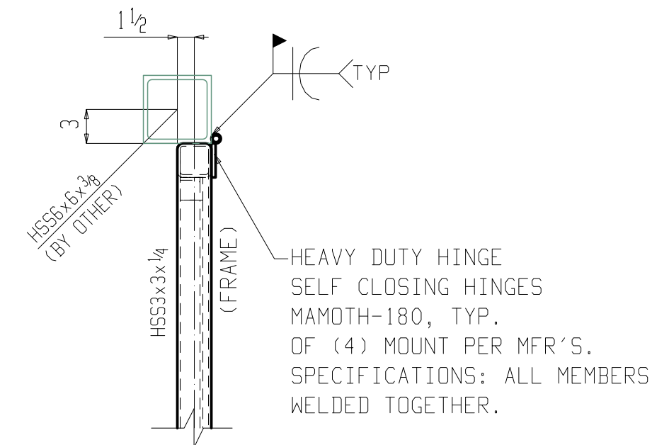
2 DETAIL VIEW ME159 (REF DWG: (E1/AS1.23))
