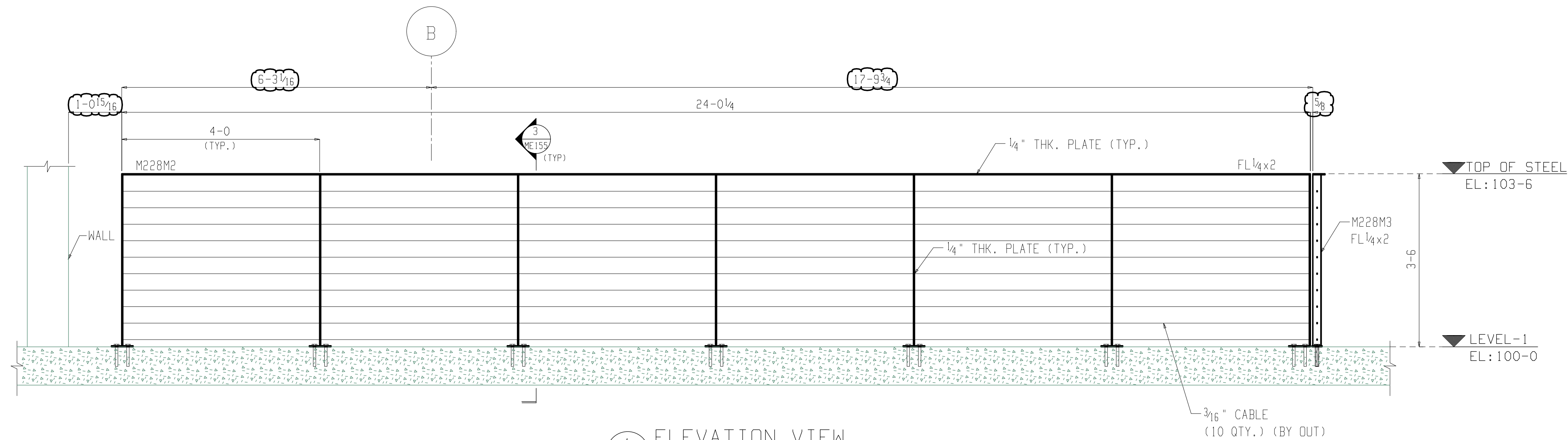
1 ELEVATION VIEW ME155
