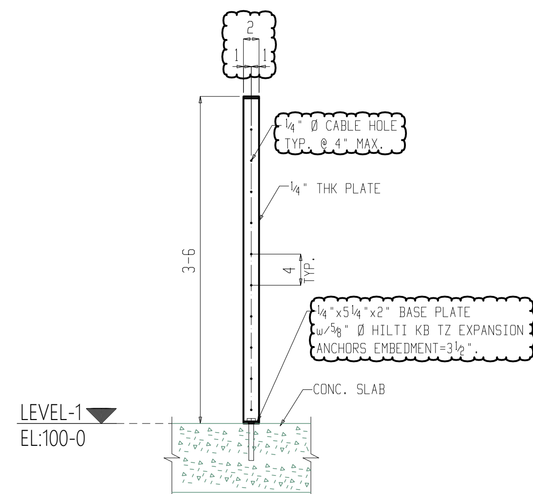
3 SECTION VIEW ME155 (REF DWG: C7/AS1.21) (FOR PCMK REFER PLAN)
