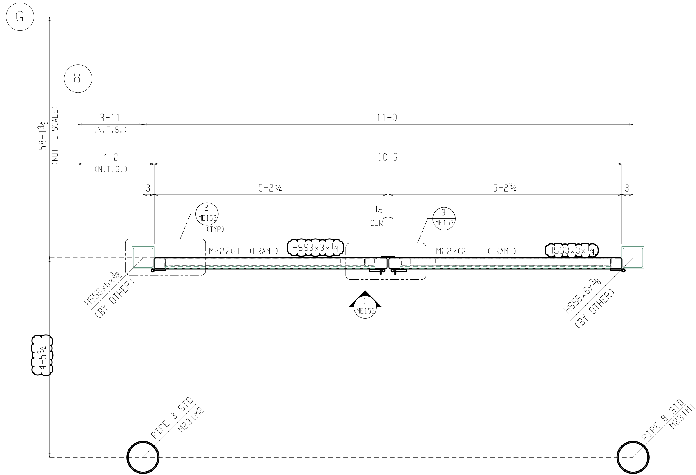
MECHANICAL ENCLOSURE GATE PLAN (REF DWG: F9/AS3.35)
