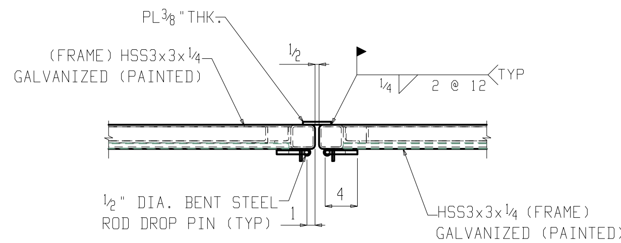
3 DETAIL VIEW ME153 (FOR PCMK REFER PLAN)
