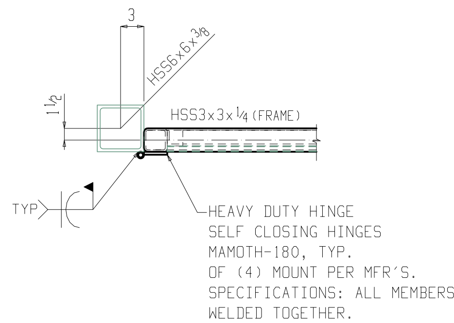
2 DETAIL VIEW ME153 (FOR PCMK REFER PLAN)
