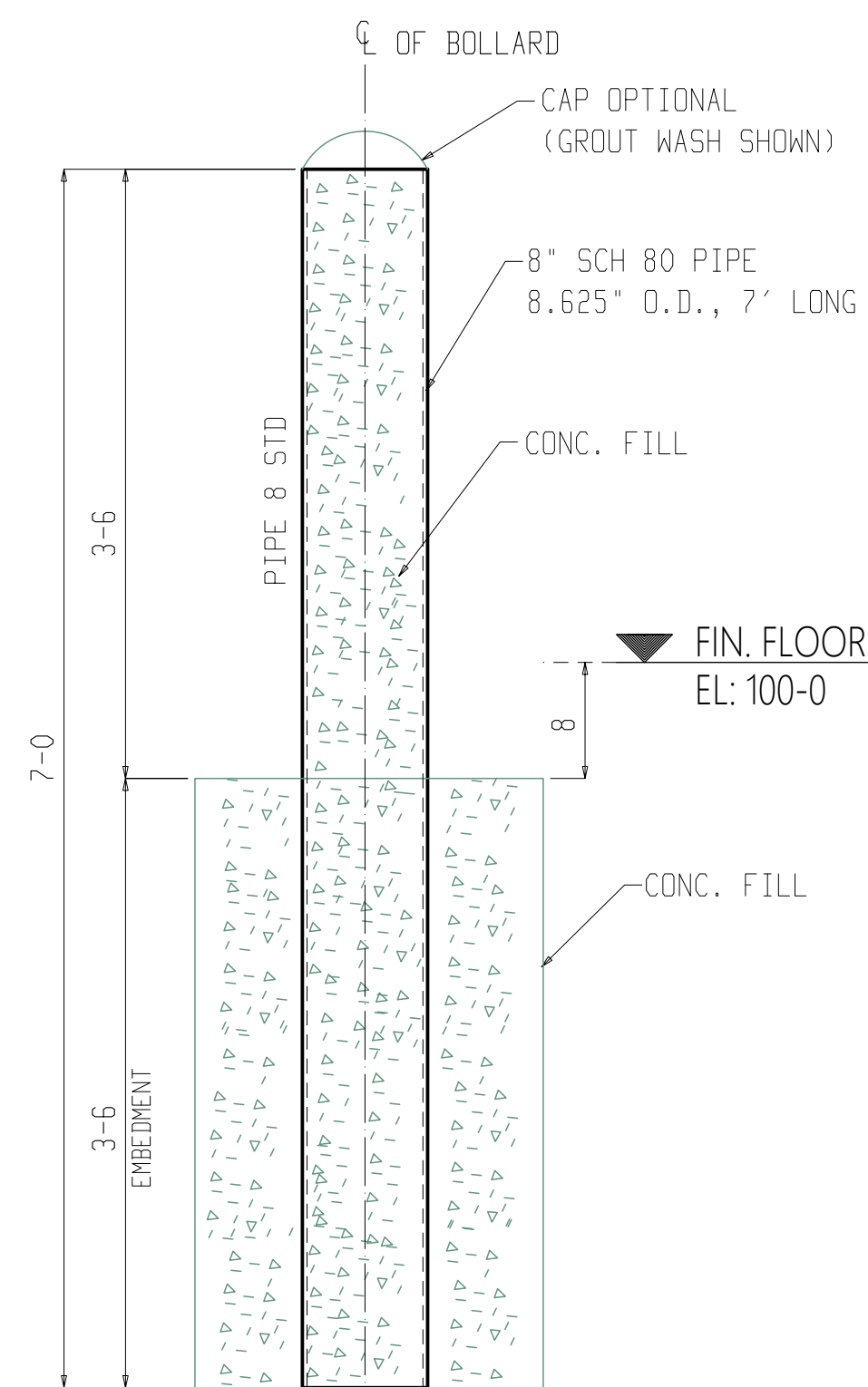
TYPICAL BOLLARD SECTION (REF. SEC.D/AS1.25)
