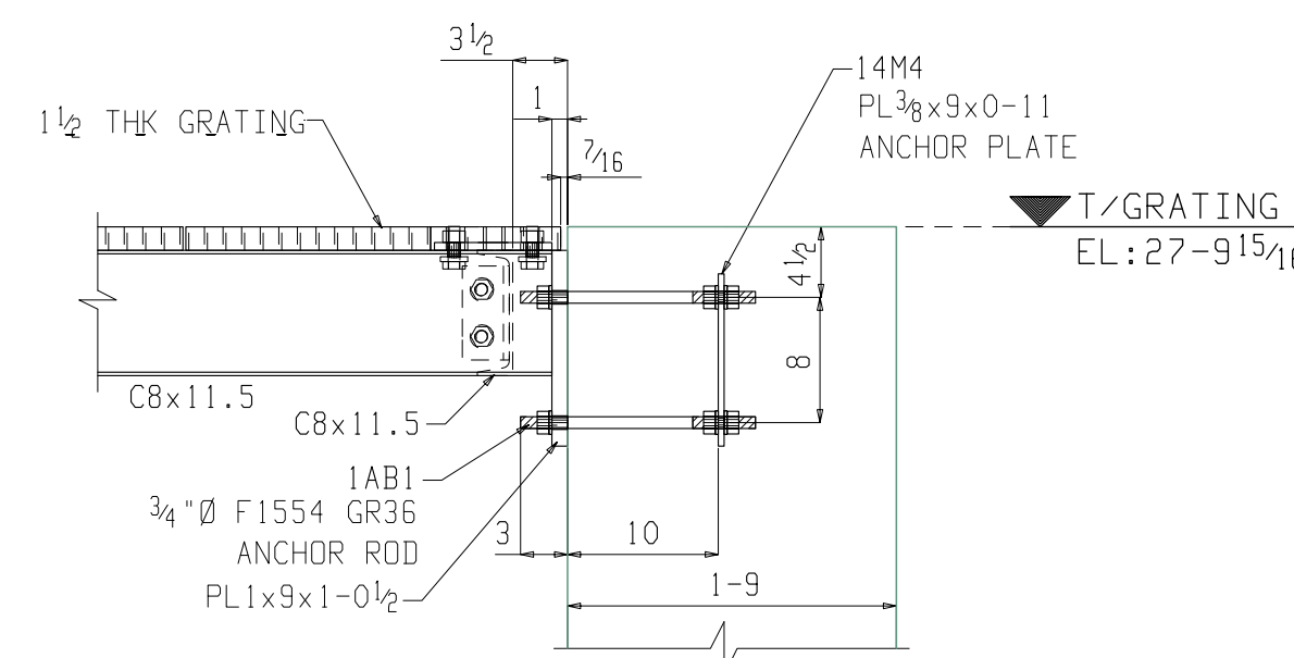
10 E3 SECTION VIEW (REF.DRW. D/A58) (HANDRAIL NOT SHOW FOR CLARITY)
