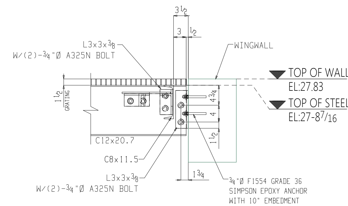
4 E3 SECTION VIEW (REF.DRW. D/A58) (HANDRAIL NOT SHOW FOR CLARITY)
