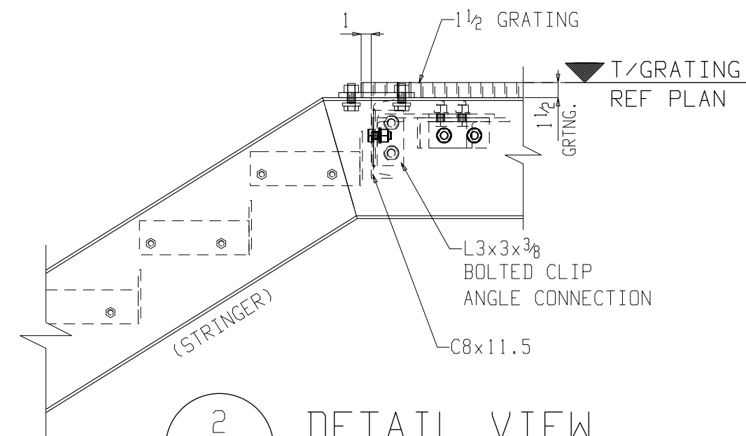
2 E2 DETAIL VIEW (REF.DRW. B/A58) (HANDRAIL NOT SHOW FOR CLARITY)
