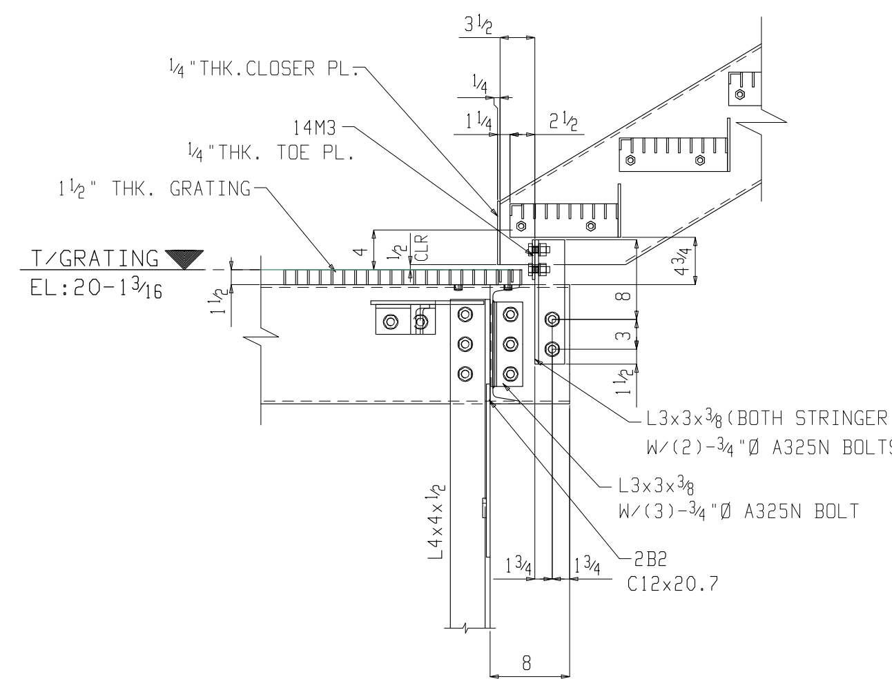
3 E3 SECTION VIEW (REF.DRW. C/A58) (HANDRAIL NOT SHOW FOR CLARITY)
