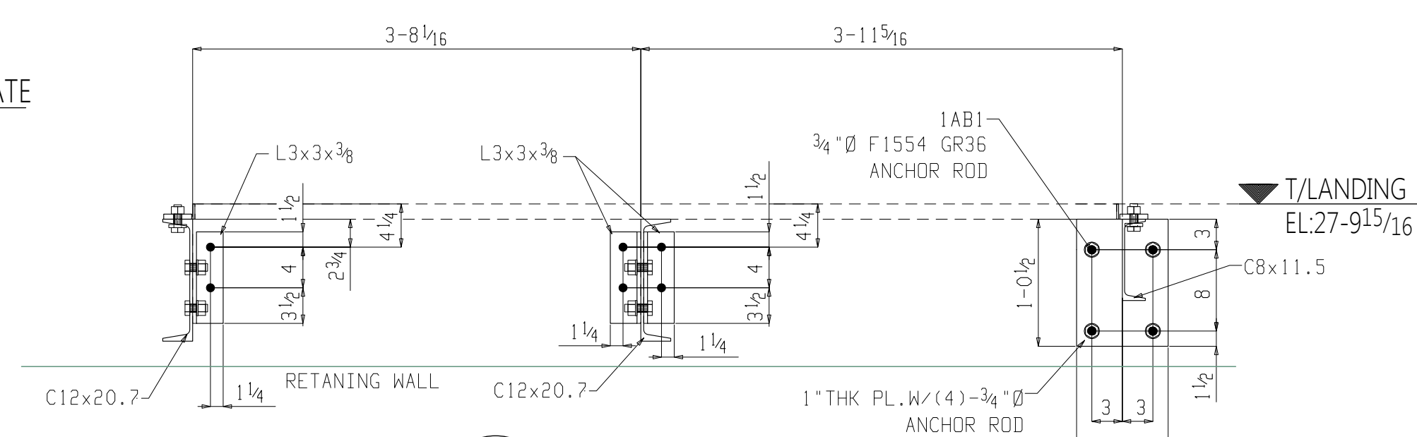
6 E3 SECTION VIEW STAIR CONNECTION TO WALL
