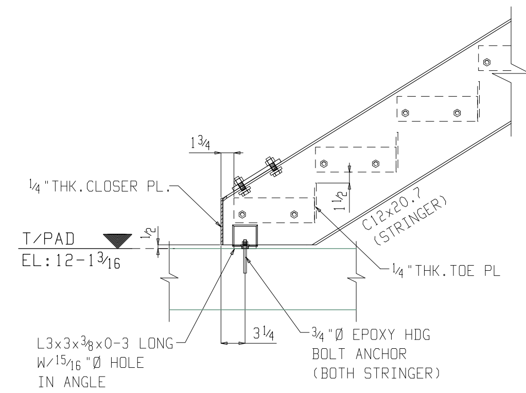
1 E3 DETAIL VIEW (REF.DRW. A/A58) (HANDRAIL NOT SHOW FOR CLARITY)
