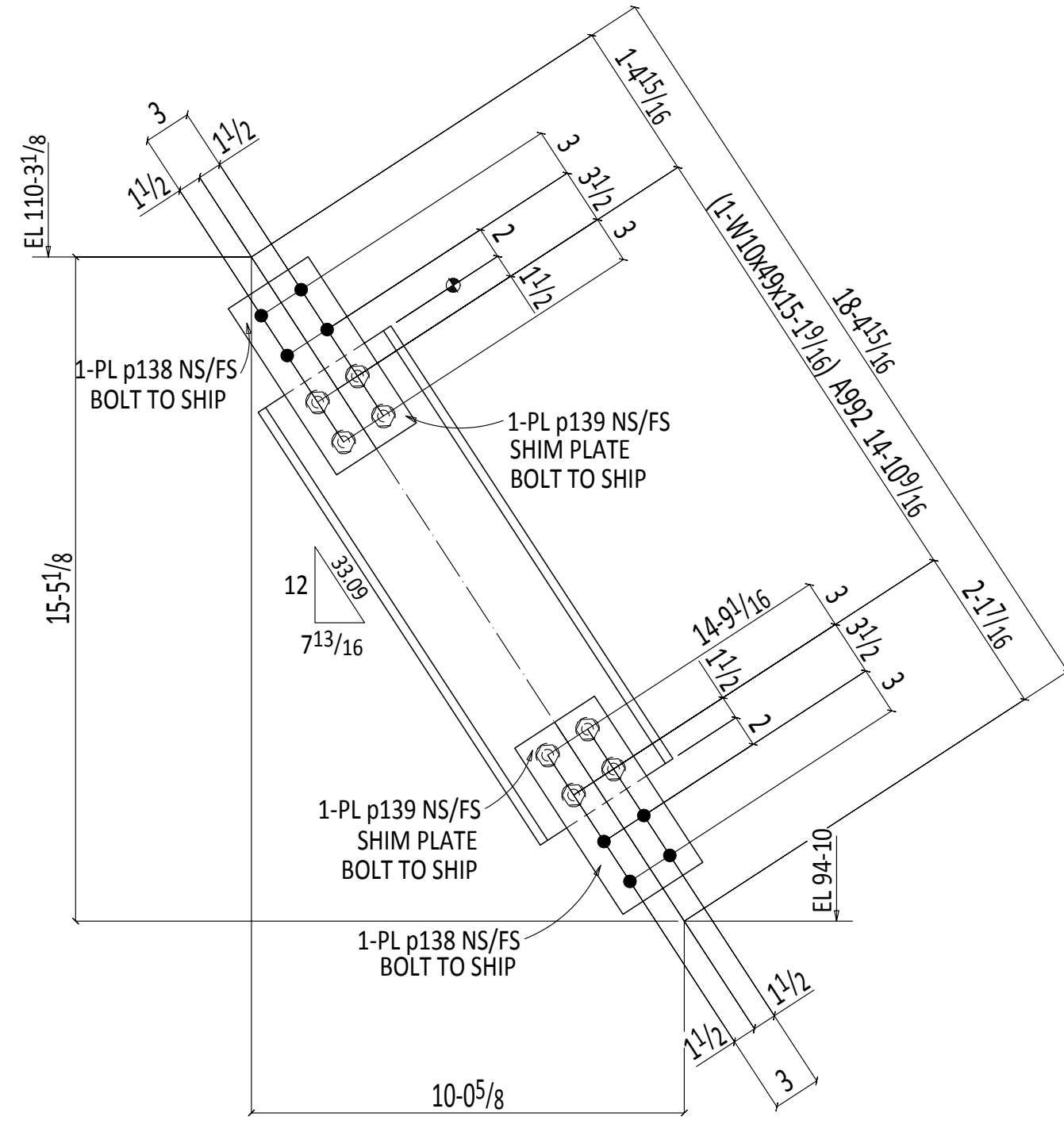
ONE VERTICAL BRACE 224VB3
