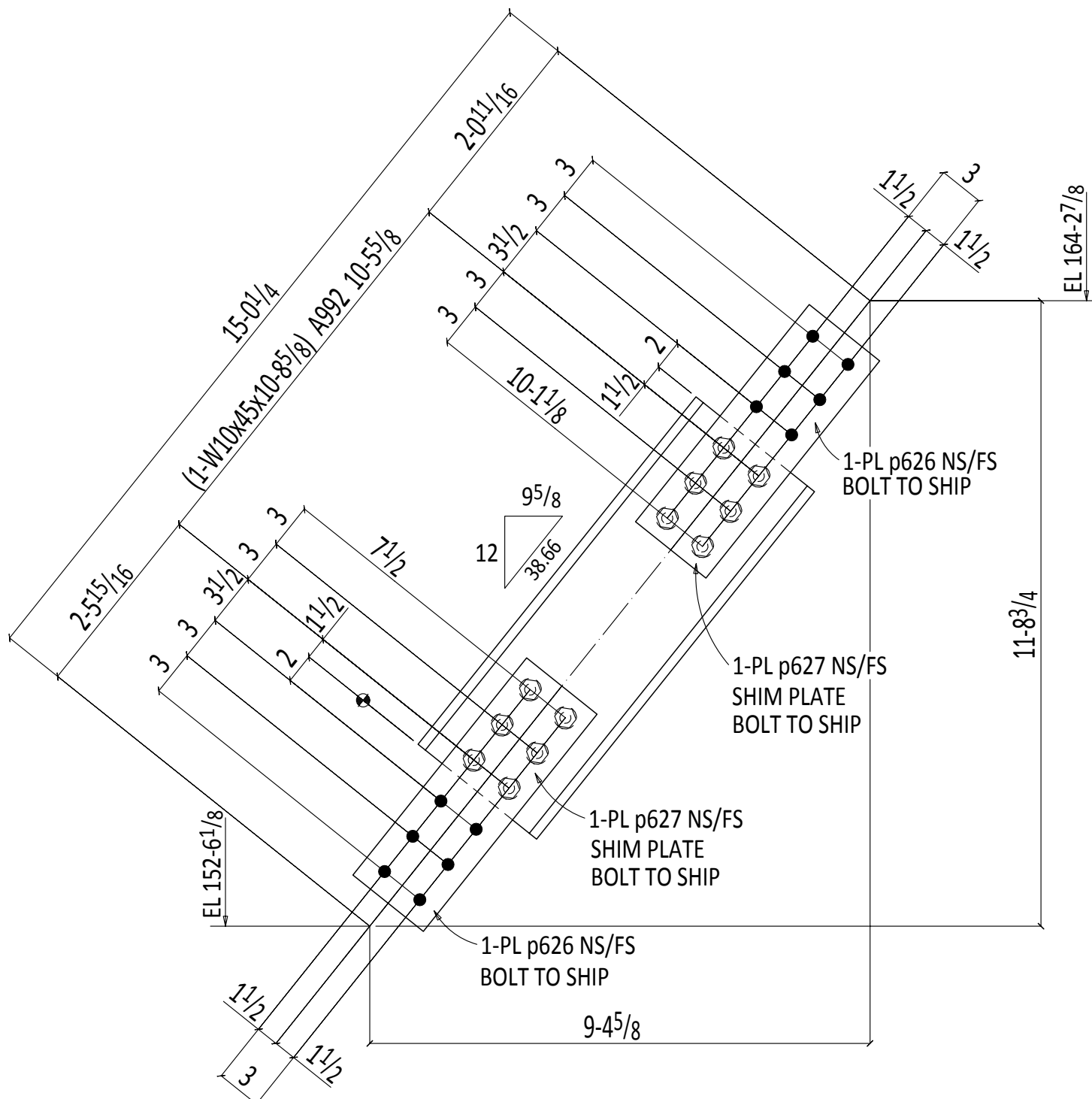
ONE VERTICAL BRACE 224VB2
