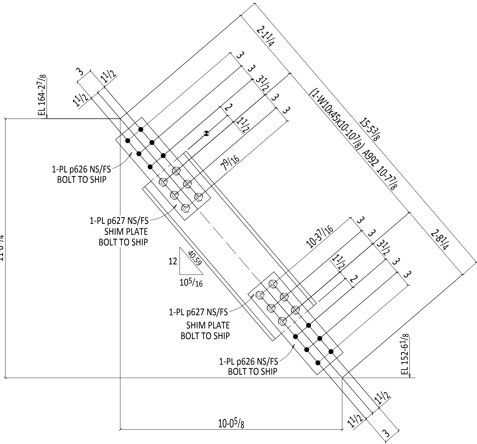
2 VERTICAL BRACES 224VB1
