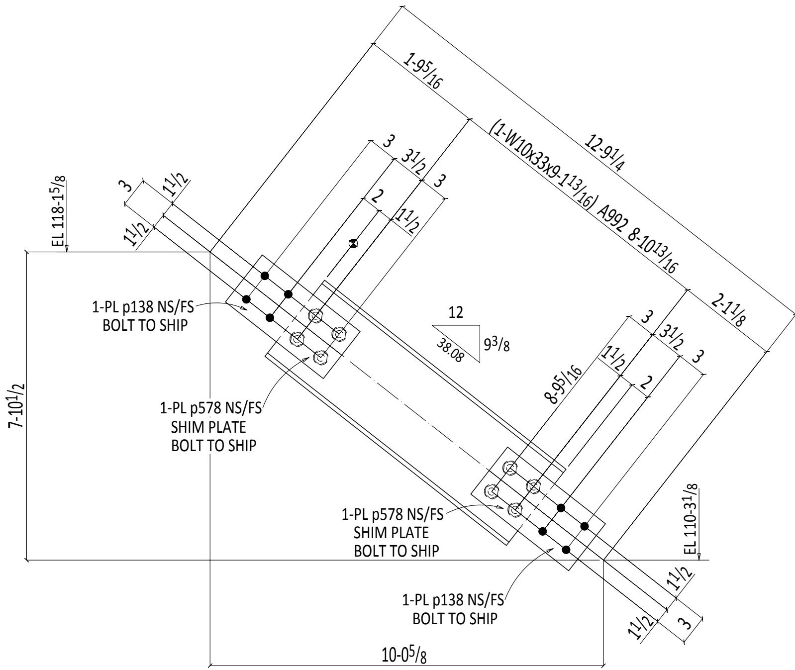
ONE VERTICAL BRACE 224VB5
