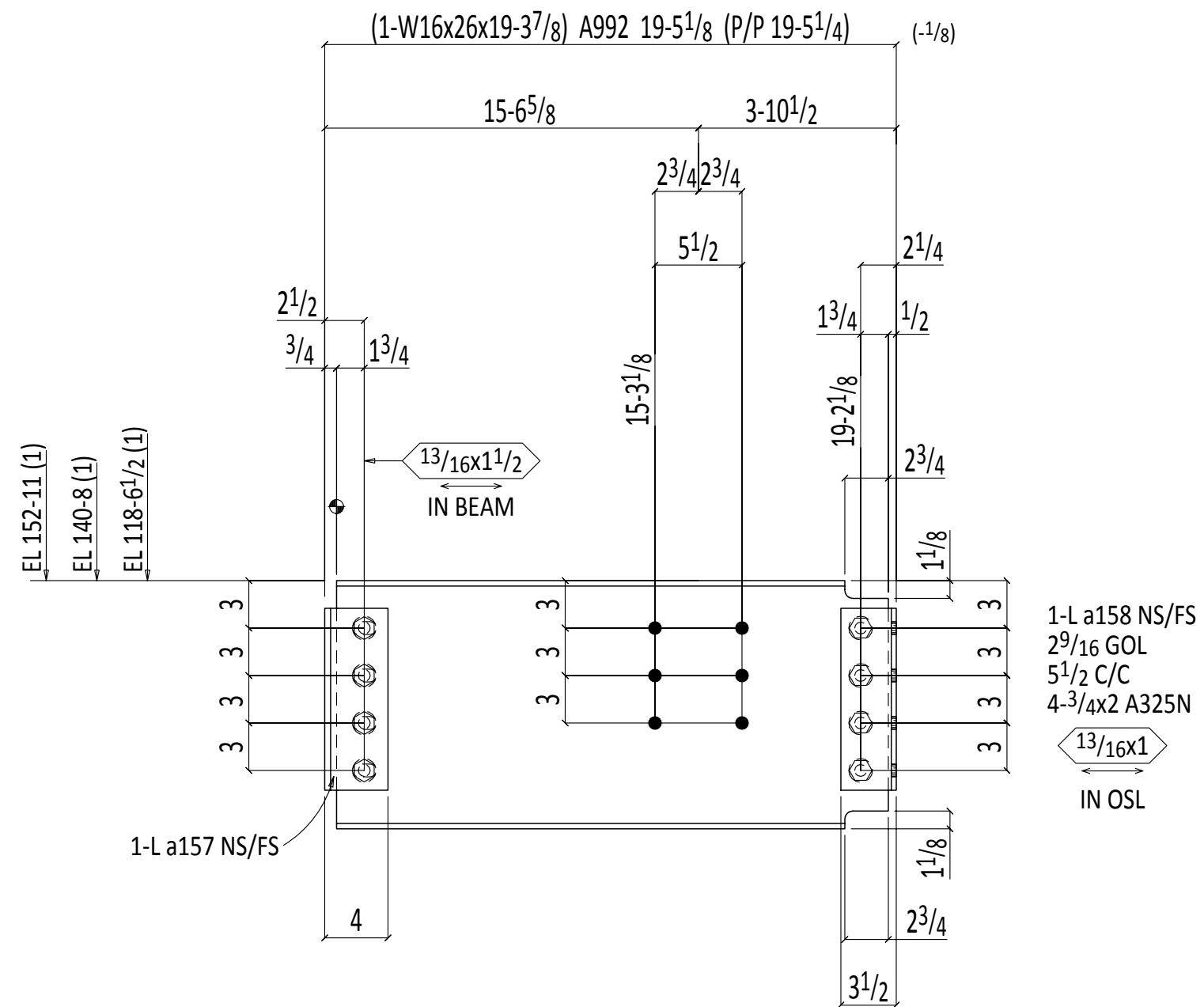
3 BEAMS 215B1
